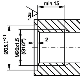
Fig.4b. Socket for P-type connector.
