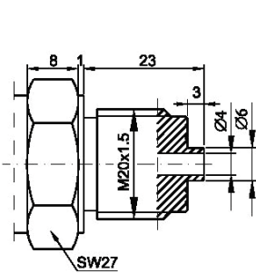
Fig.3a. M-type connector with M20x1.5 thread
